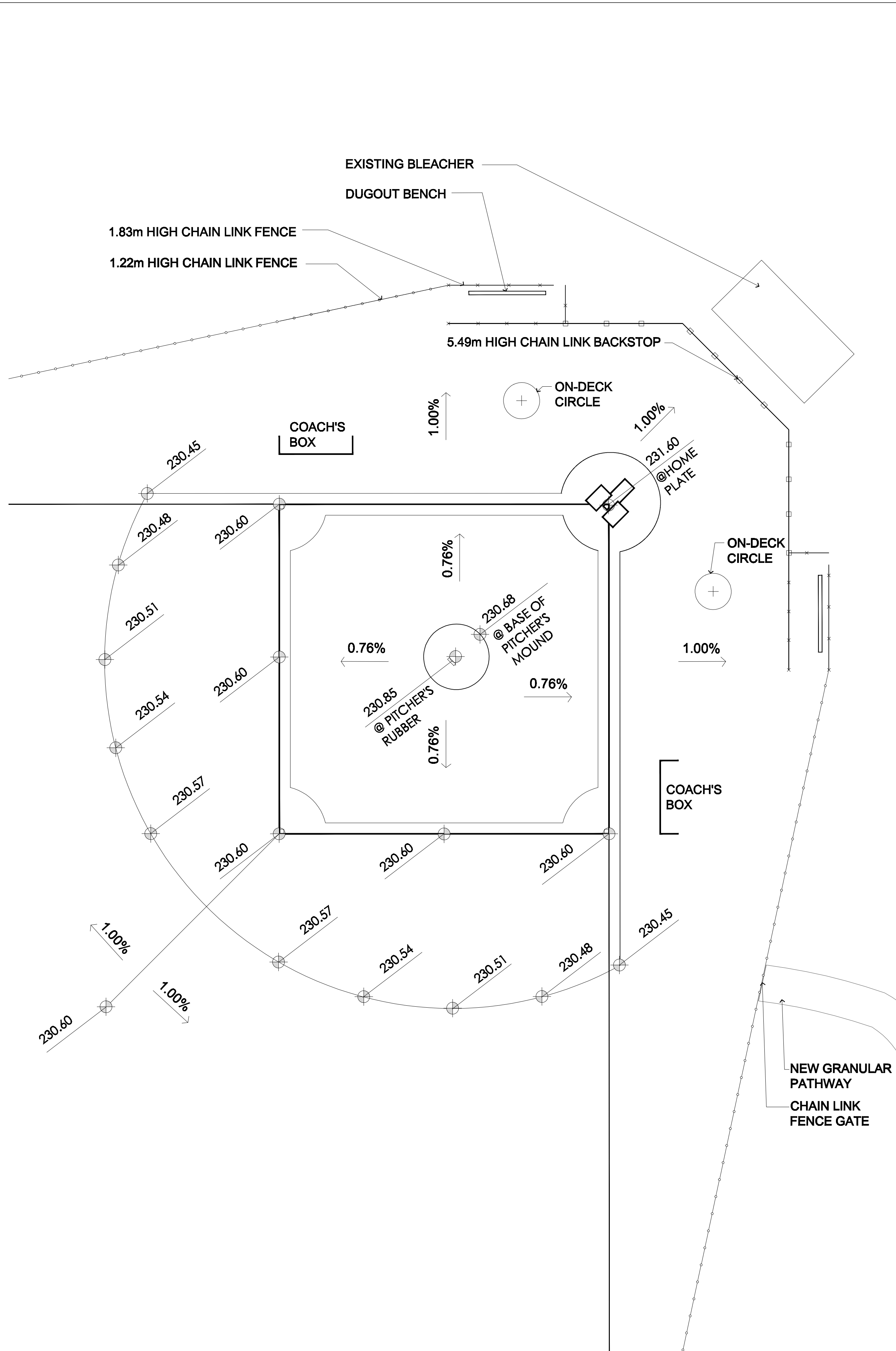
BASEBALL DIAMOND GRADING DETAILS Scale 1:200
