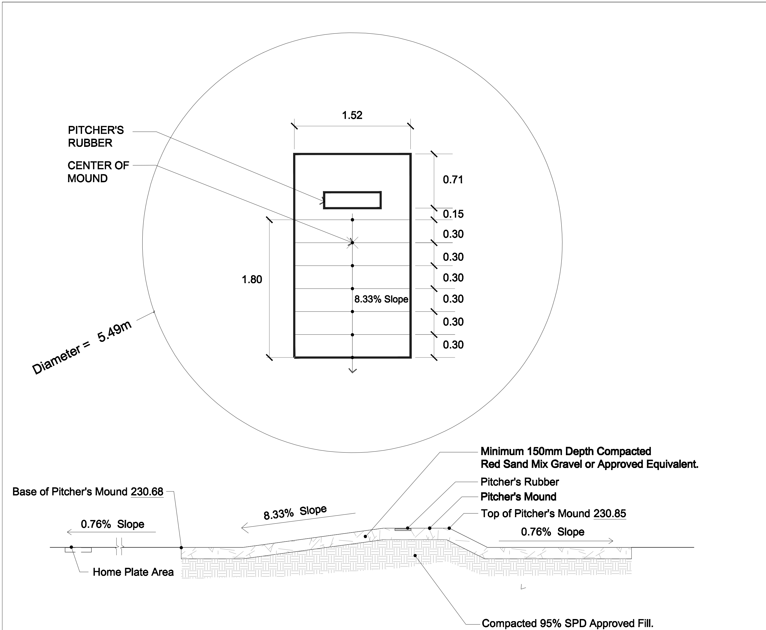
PITCHER'S MOUND DETAILS Scale 1:25
