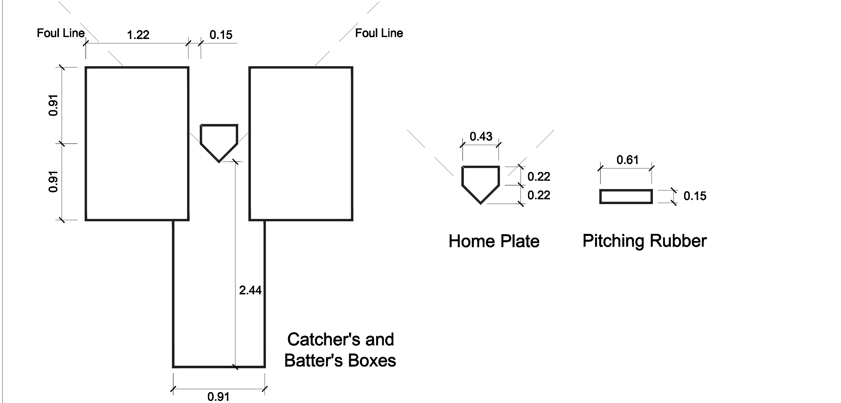
CATCHER'S AND BATTER'S BOXES, HOME PLATE AND PITCHING PLATE DIMENSIONS Scale 1:25
